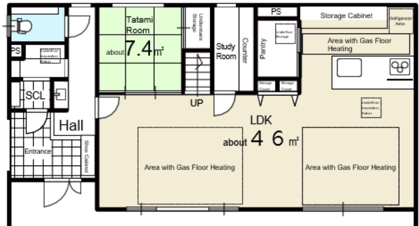
1st-Floor Layout
